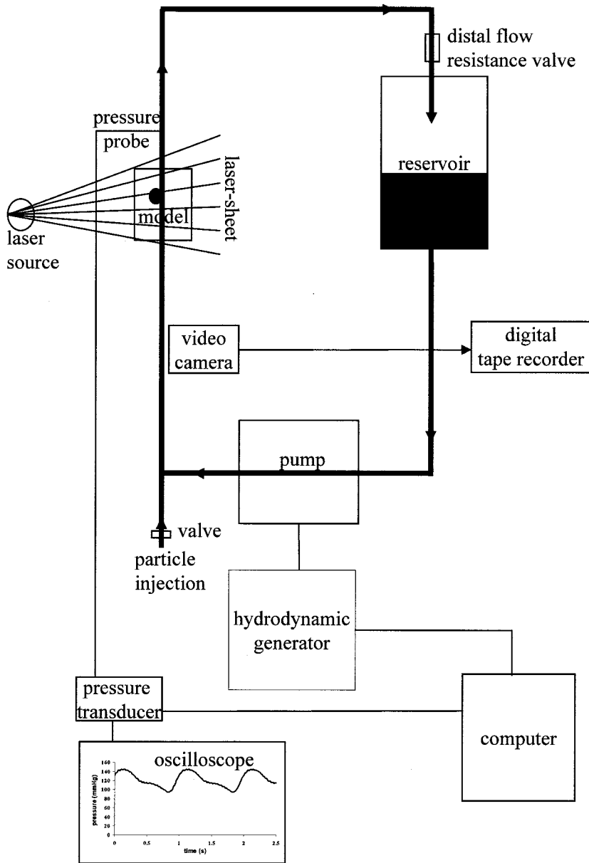
FIG 3. Experimental setup.
